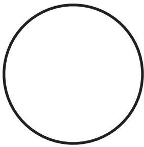
A. First Quarter
