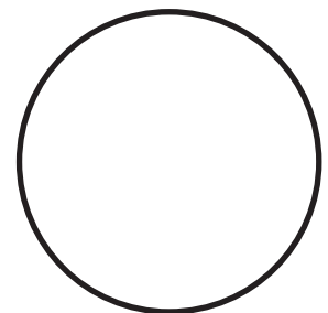
H. Waxing Crescent
